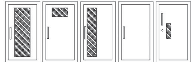
F - Full glass with pull handle D - Horizontal duo panel with pull handle V - Vertical duo panel with pull handle S21 - Solid with pull handle B - Small view window with pull handle G - Full glass with pull handle above Saf-T-Lok (Not Shown) E - Horizontal duo panel with pull handle above Saf-T-Lok. (Not Shown) W - Vertical duo panel with pull handle above Saf-T-Lok. (Not Shown) S21 - Solid with pull handle above Saf-T-Lok L24 - Solid with cylinder key lock and no handle (Not Shown) L22 - Solid with pull handle, above Saf-T-Lok
